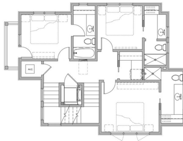
Second Level
