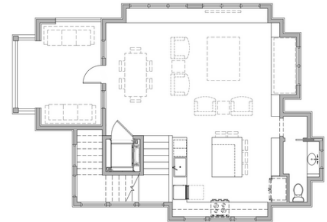
Third Level
